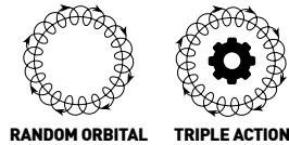
RANDOM ORBITAL
