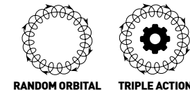
RANDOM ORBITAL
